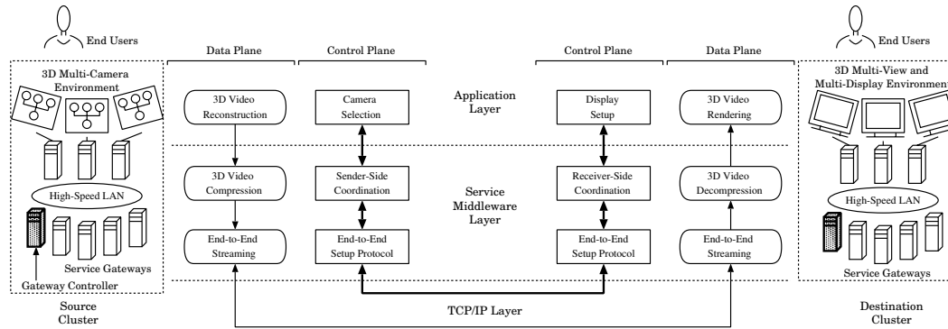
Figure 4: TEEVE Architecture
