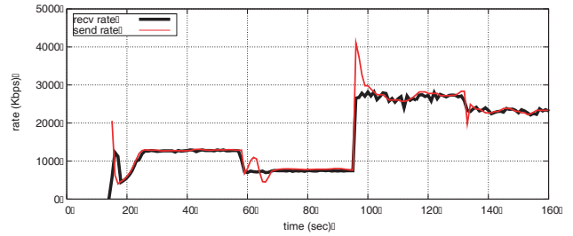
Fig. 6. Multi-rate scenario with one flow.
