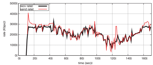
Fig. 7. Multi-rate scenario (mobile).
