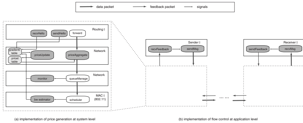
Fig. 3. Software Architecture for Joint Flow Control and Active Queue Management.
