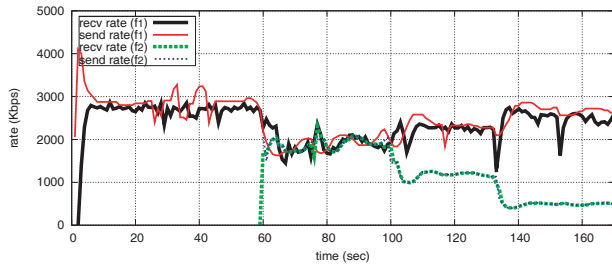
Fig. 8. Multi-rate scenario with two flows.
