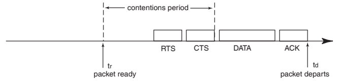
Fig. 4. Measurement-based bandwidth estimation.
